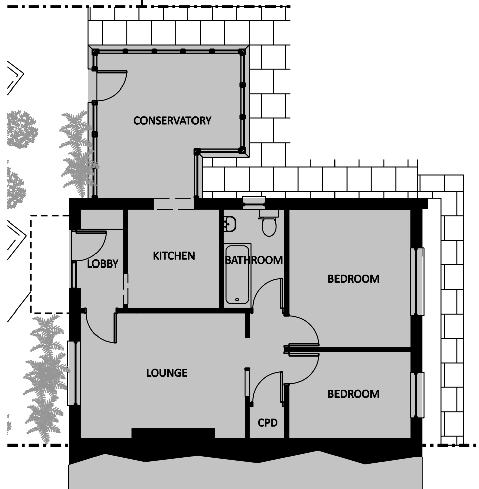
PROPOSED GROUND FLOOR PLANS
